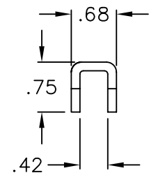
BUTT SPLICE BRACKET
