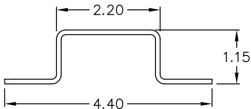
CEILING SUPPORT BRACKET
